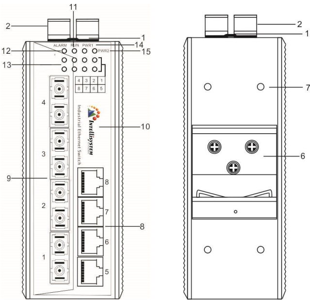
Front panel
