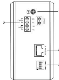
Bottom Panel
